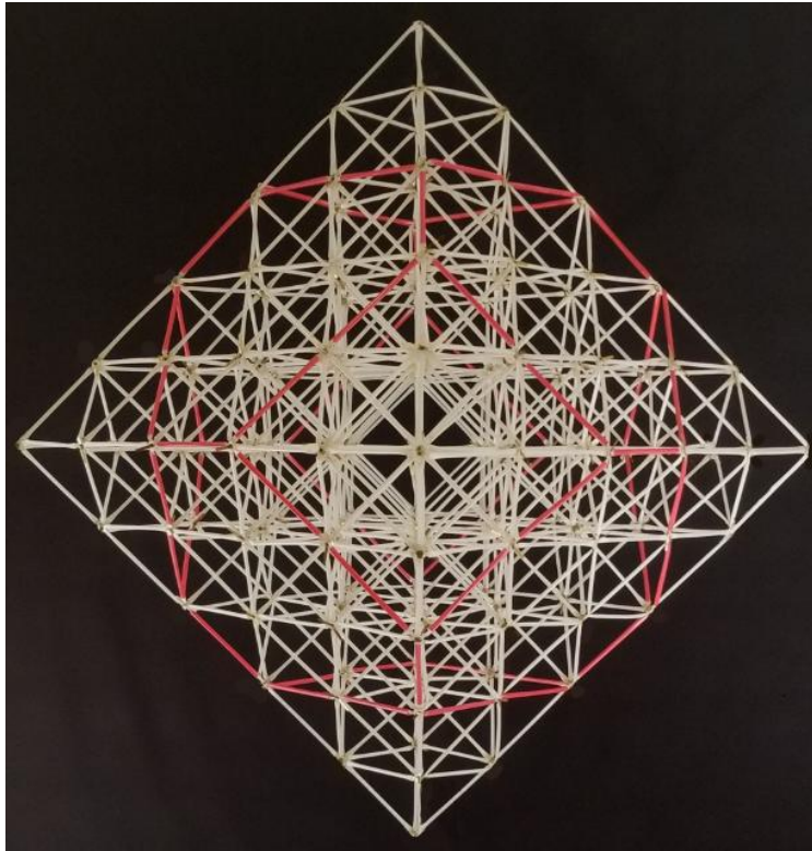
Figure J1: Truncating a Large Octahedral-Tetrahedral Lattice
