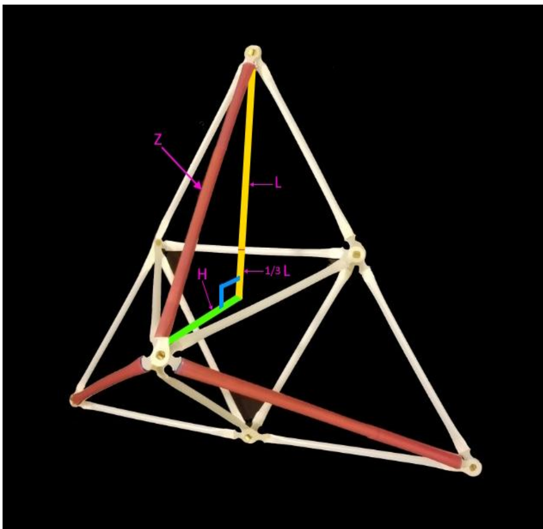
Figure Q8: Great Triangle with Tetrahedron at Center and Three Lines to Outer Nodes
