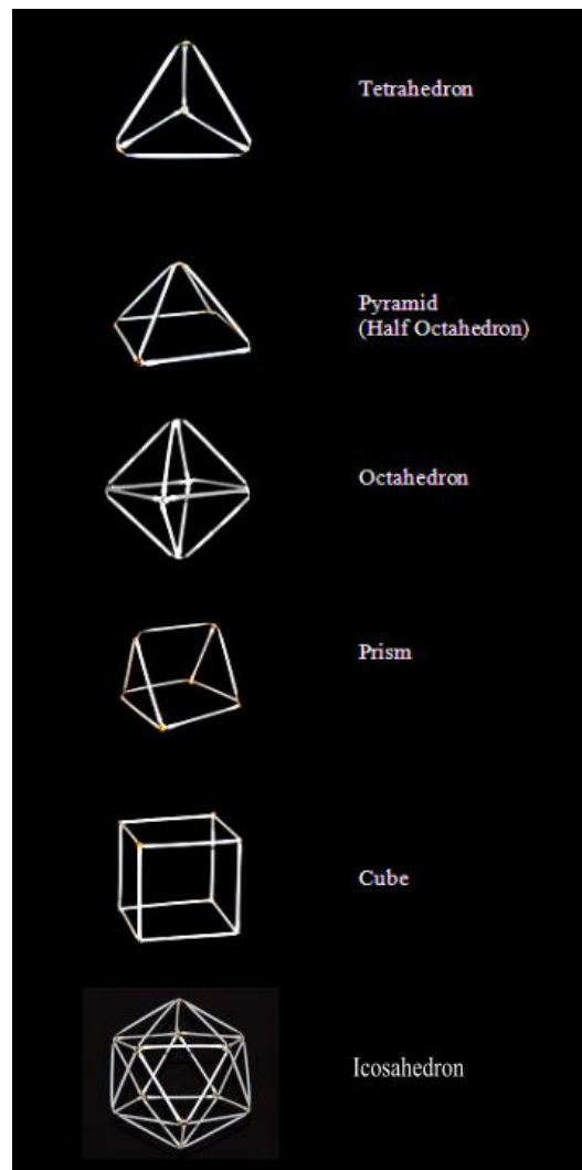
Figure C1: Base Forms of Triangle and/or Square
