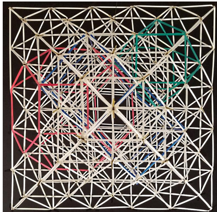
Figure R2: Cube, Cuboctahedron and Truncated Octahedron Sub-Forms: Vertex View
