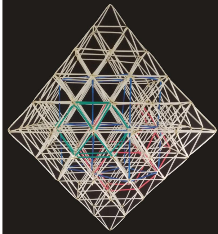
Figure R1: Cube, Cuboctahedron and Truncated Octahedron Sub-Forms: Edge View
