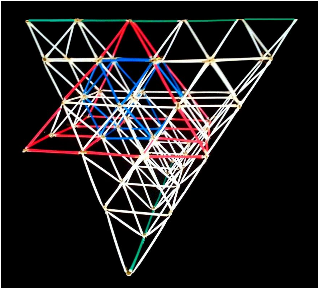
Figure C9: Octahedral-Tetrahedral Lattice with VE aspect highlighted
