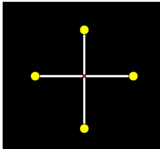
Figure A8: View of Tetrahedron nodes looking from mid-point of one line to its opposite
