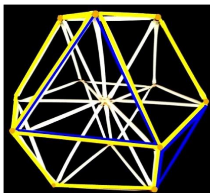
Figure E10: Mated Facets of Triangle-at-Center (Cuboctahedron)
