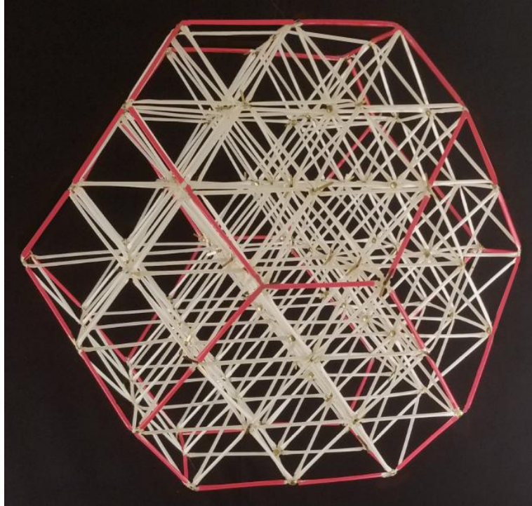
Figure J2: The Form of the Second Expansion of Cuboctahedron
