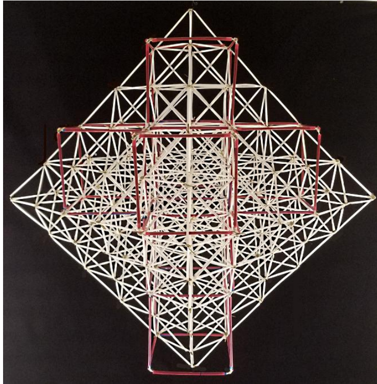
Figure Q2: \sqrt{2} Cubic Lattice Aspect – Looking at Octahedron Vertex 14
