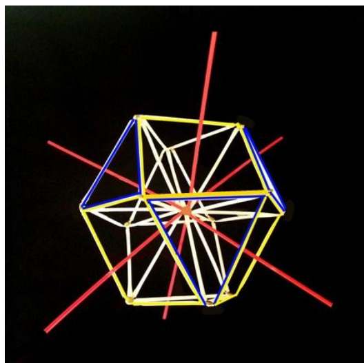
Figure C10: Orthogonal Square Faces of the VE
