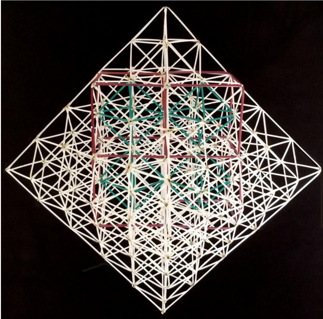
Figure Q6: Octahedral-Tetrahedral Lattice as a stacking of \sqrt{2} Cubes
