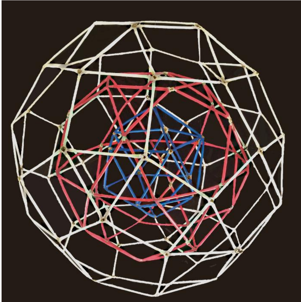
Figure E2: Icosahedral Expansion Sequence
