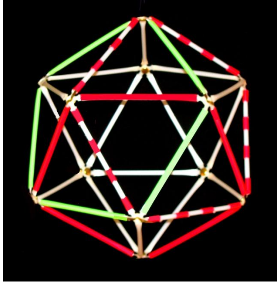
Figure D5: Enmeshed Pentagons of the Icosahedron
