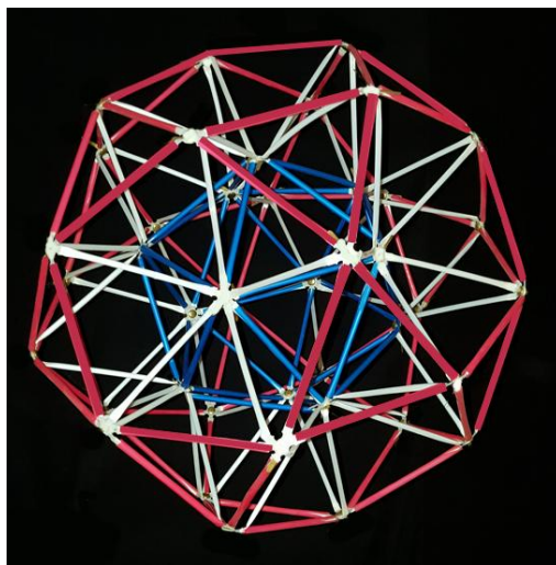
Figure D3: Model of First Cage Layer 6
