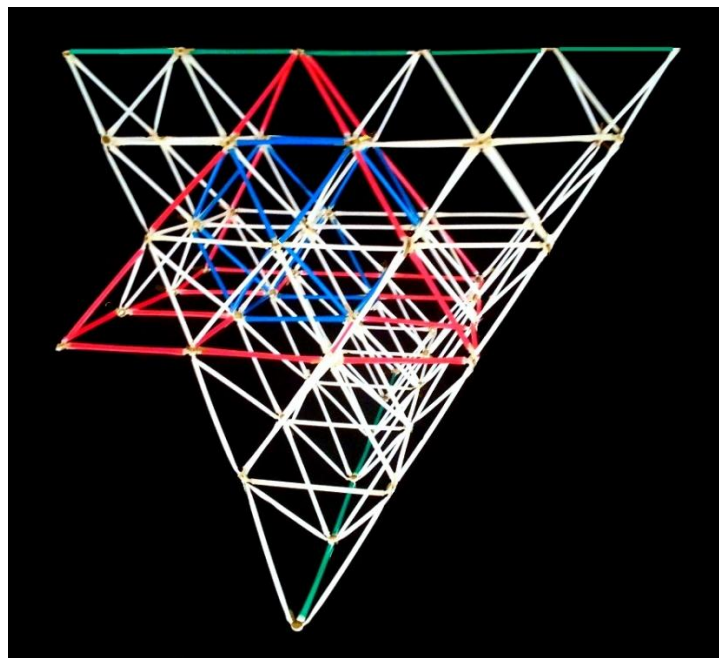
Figure C9 (copy) – The 3D Octahedral-Tetrahedral Lattice
